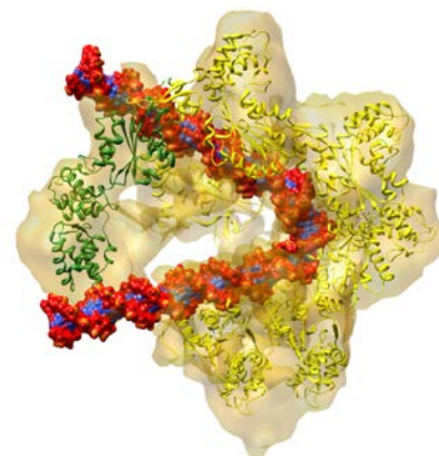
Cryo-EM can be used to determine the structures of large molecular complexes such as the origin recognition complex (ORC). The ORC recognizes and binds DNA to start the process that copies the cell's genetic material prior to cell division. Credit: Huilin Li, Brookhaven National Laboratory, and Bruce Stillman, Cold Spring Harbor Laboratory.
