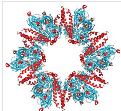
A mix of alpha helices (red; curled ribbon forming a six-sided star) and beta sheets (blue; thinner, tangled strands). Credit: RCSB Protein Data Bank.
