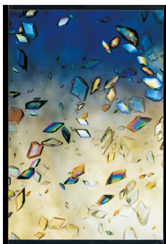
Structural biologists create crystals of proteins, shown here, as a first step in X-ray crystallography, which can reveal detailed, three-dimensional protein structures. Credit: Alex McPherson, University of California, Irvine.
